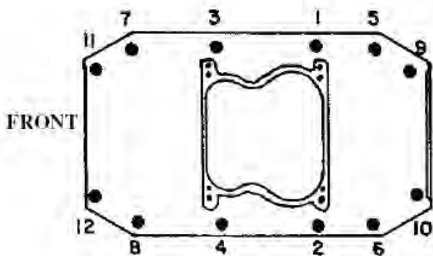
Figure 1 Intake Manifold Tightening Sequence
